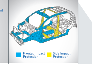
Collision-resistant Body
